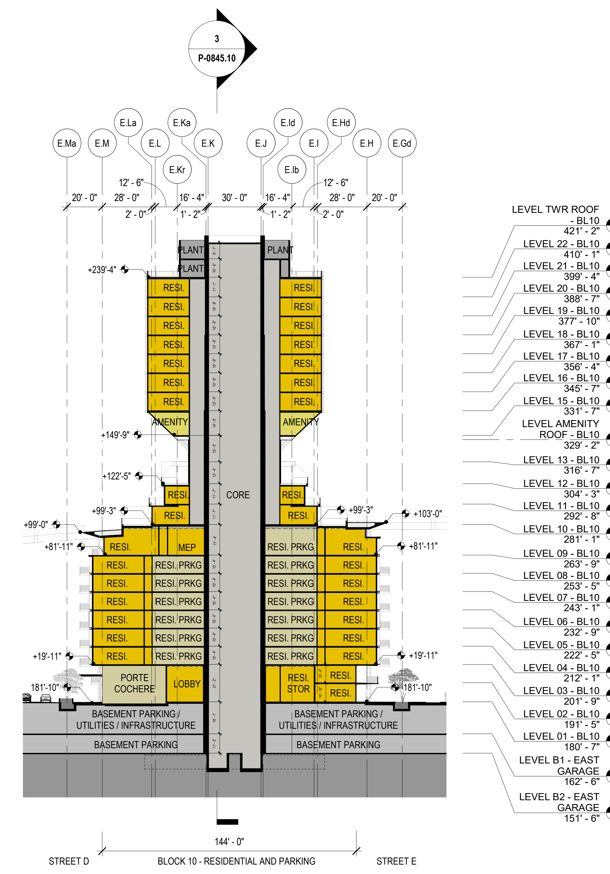
BLOCK 10 - CROSS SECTION 1/32" = 1'-0"
