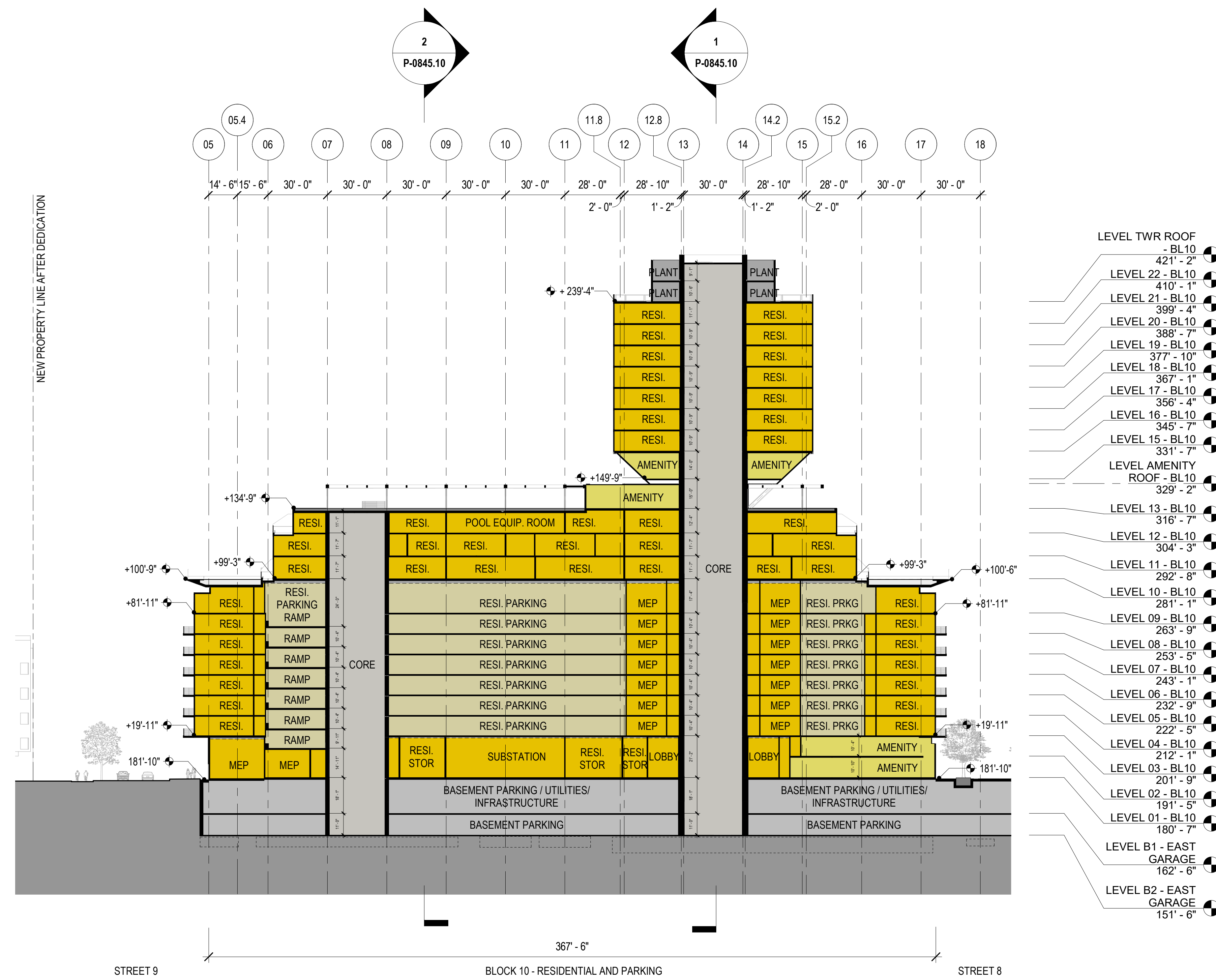
BLOCK 10 - LONGITUDINAL SECTION 1/32" = 1'-0"
