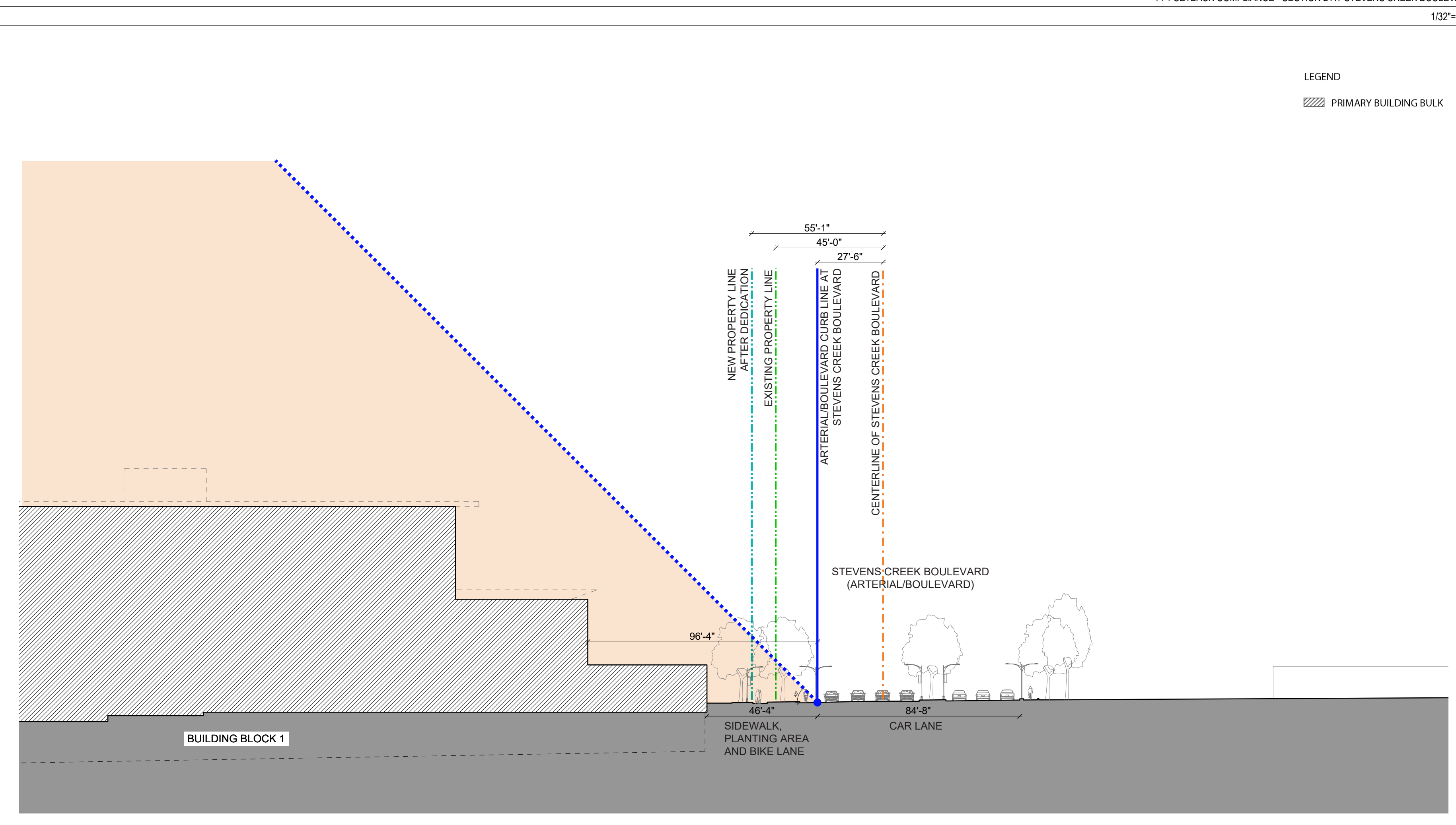
1:1 SETBACK COMPLIANCE - SECTION 3 AT STEVENS CREEK BOULEVARD 1/32"=1'-0"
