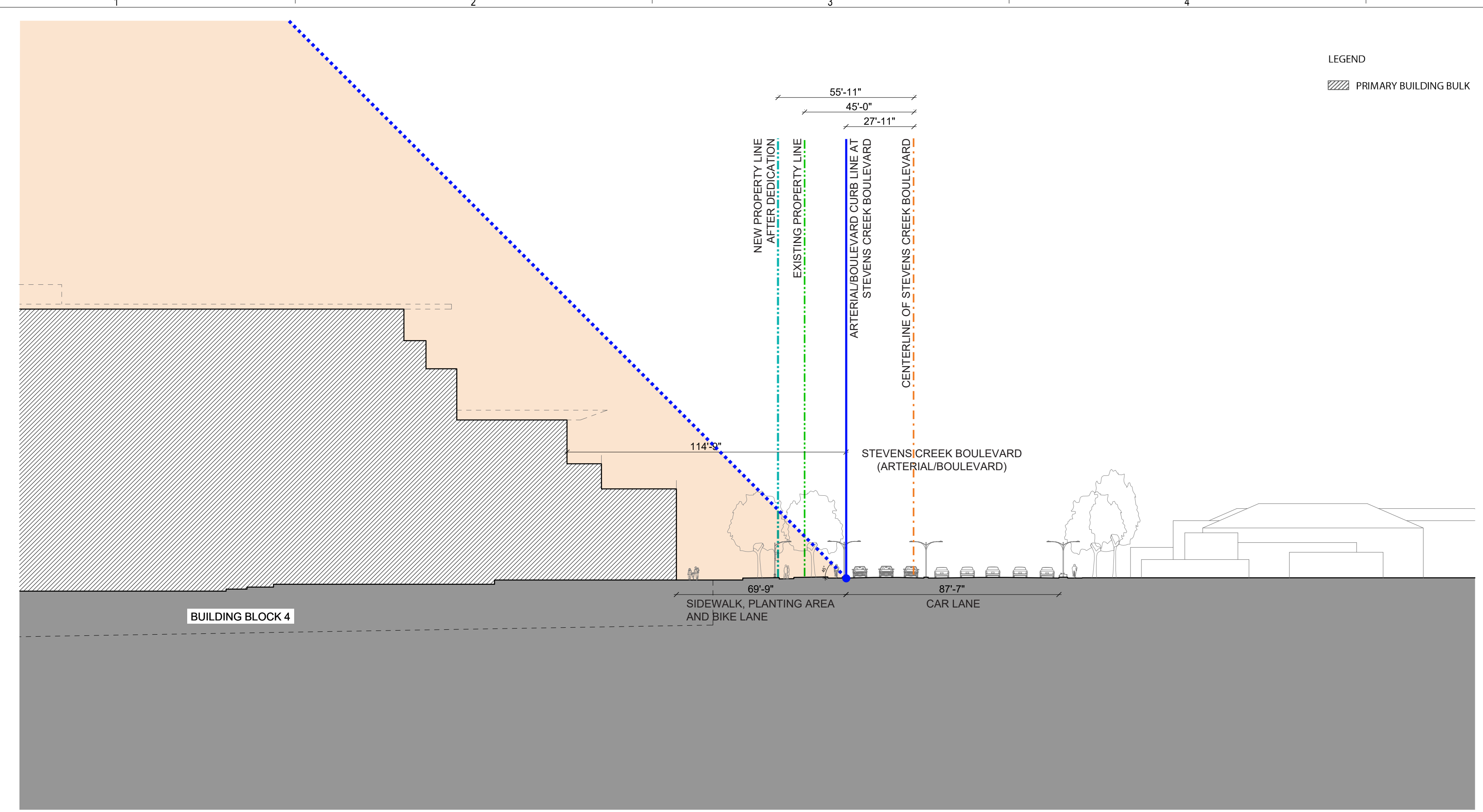
1:1 SETBACK COMPLIANCE - SECTION 1 AT STEVENS CREEK BOULEVARD 1/32"=1'-0"
