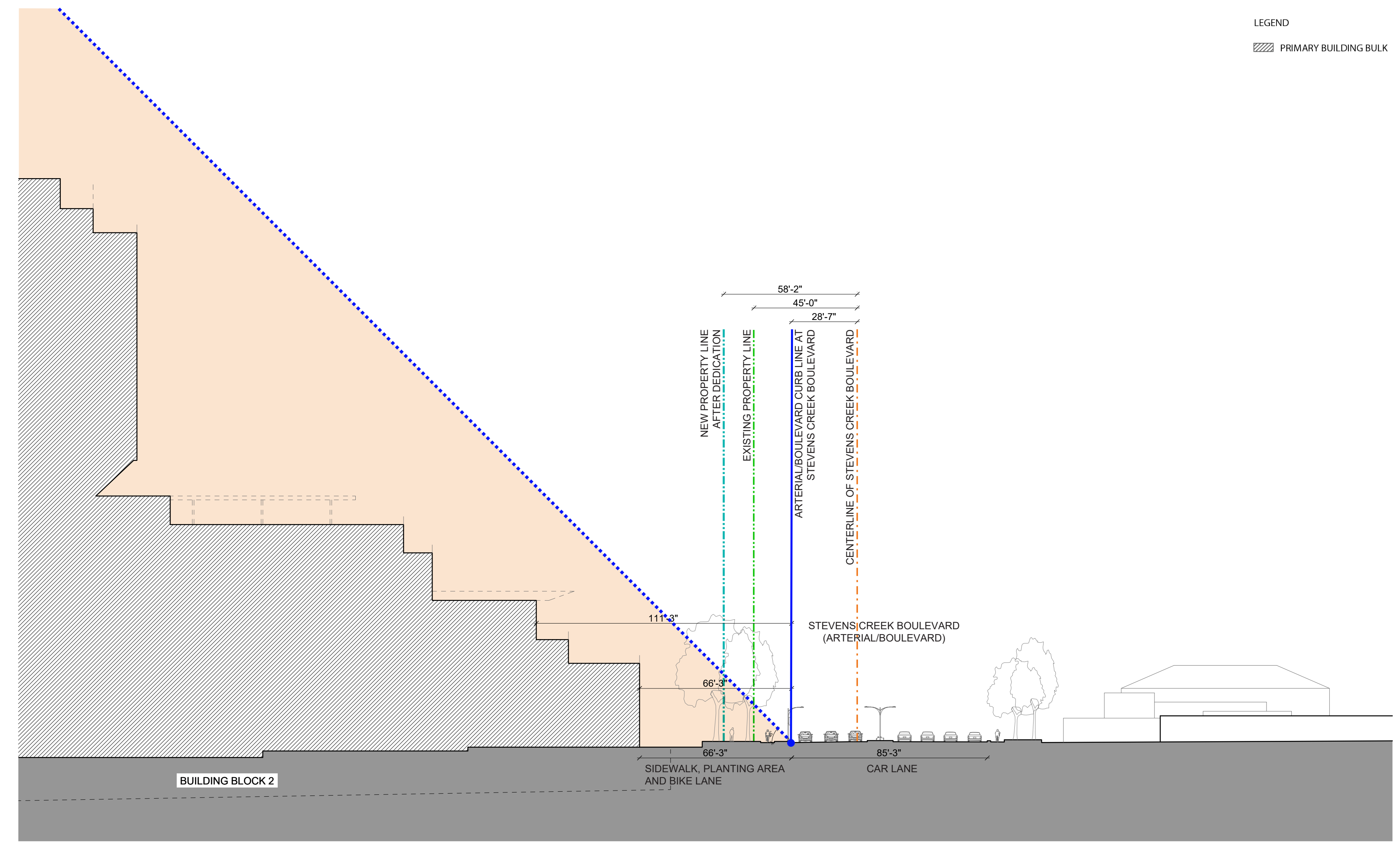
1:1 SETBACK COMPLIANCE - SECTION 2 AT STEVENS CREEK BOULEVARD 1/32"=1'-0"
