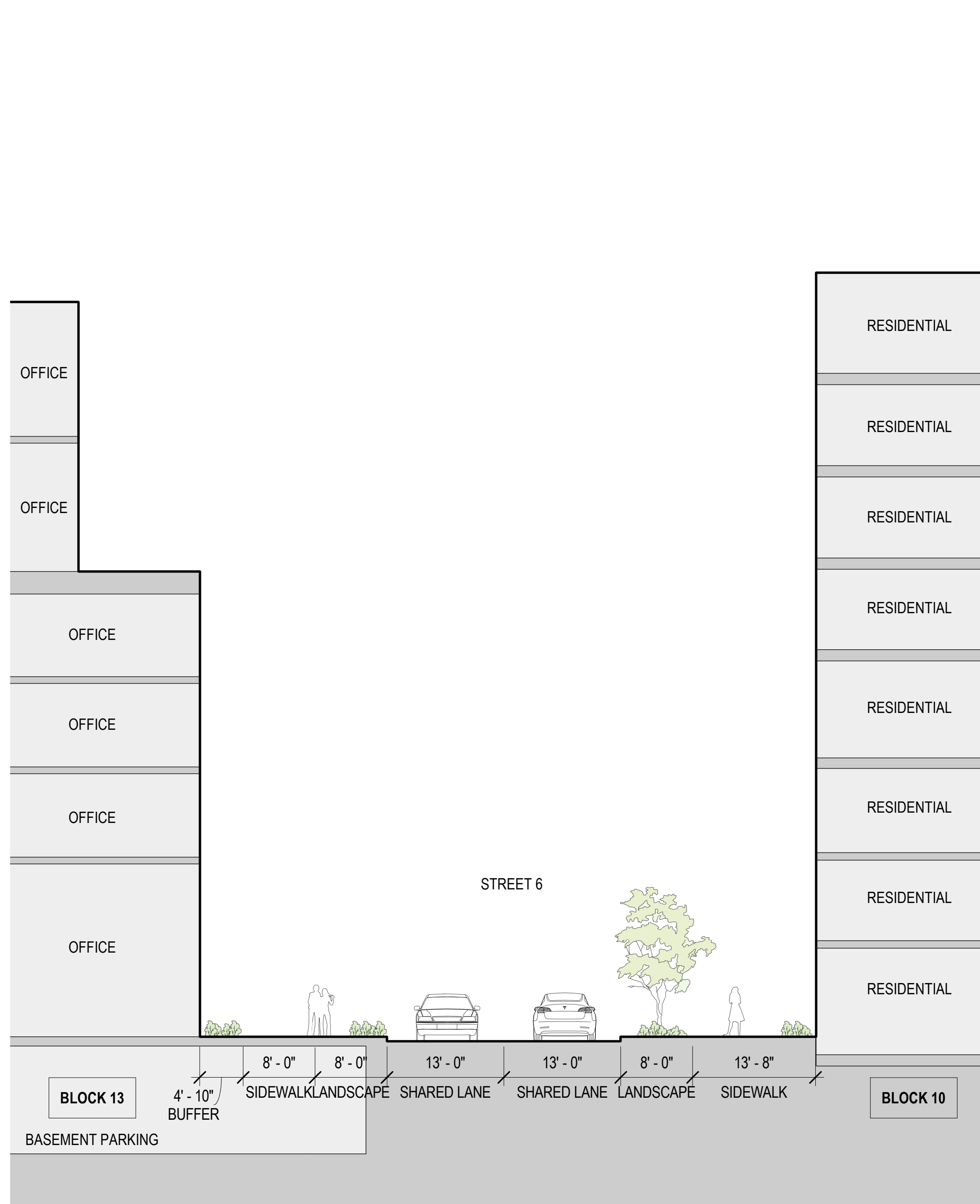
2 STREET SECTION STREET 6 - BLOCKS 10 & 13 SCALE: 1" = 10'-0"
