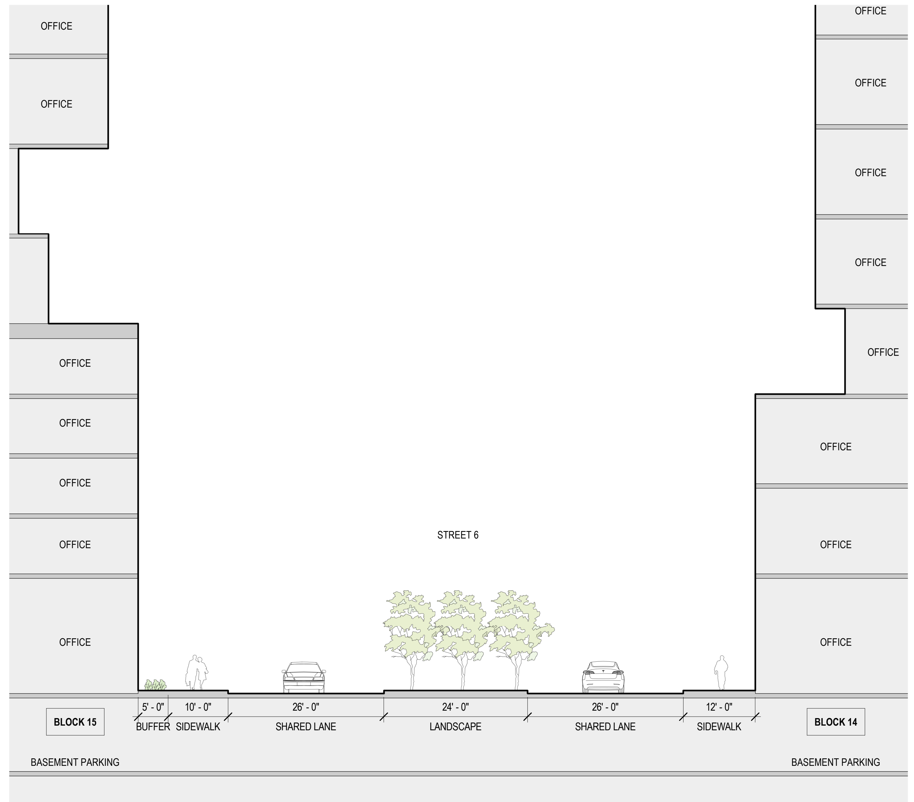
3 STREET SECTION STREET 6 - BLOCKS 14 & 15 SCALE: 1" = 10'-0"
