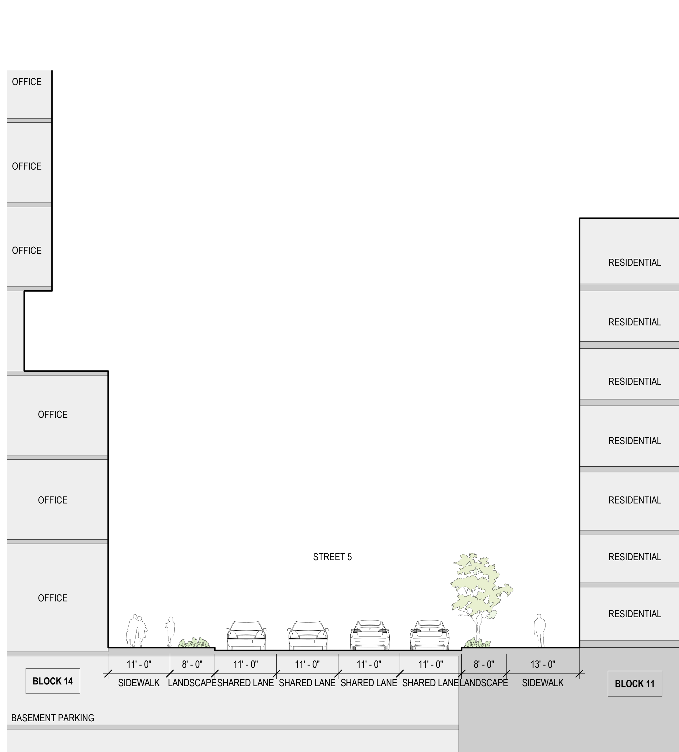
1 STREET SECTION STREET 5 - BLOCKS 11 & 14 SCALE: 1" = 10'-0"
